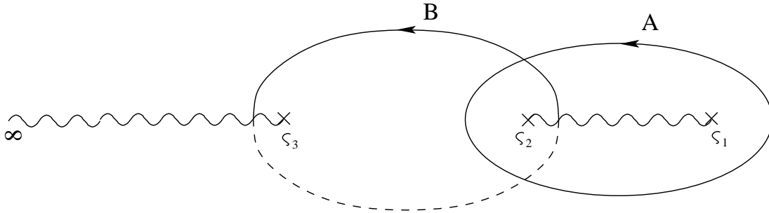
Figure 2: The cut sphere. The two cuts, drawn as wavy lines, are between \varsigma_1 and \varsigma_2 and between \varsigma_3 and \infty . We have drawn two independent nontrivial closed curves. The curve A doesn't cross any cut, so it remains on the top sheet. The curve B however, crosses the cut between \varsigma_3 and \infty , where it goes to the lower sheet (it is then drawn with a dashed line). It then crosses the other cut and comes back to the top sheet.
